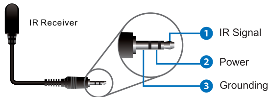
IR RECEIVER
