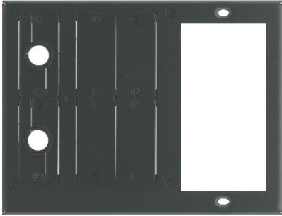
Figure 1: T1AF-26 Inner Frame (P/N: 80-000399)
