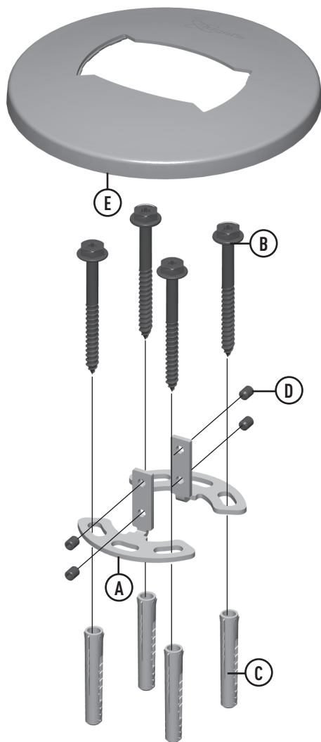
PFA 9103 Floor plate
