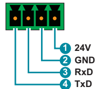
RS-232 Port 2 (HDBaseT extension)
