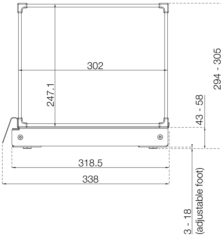
Side view
